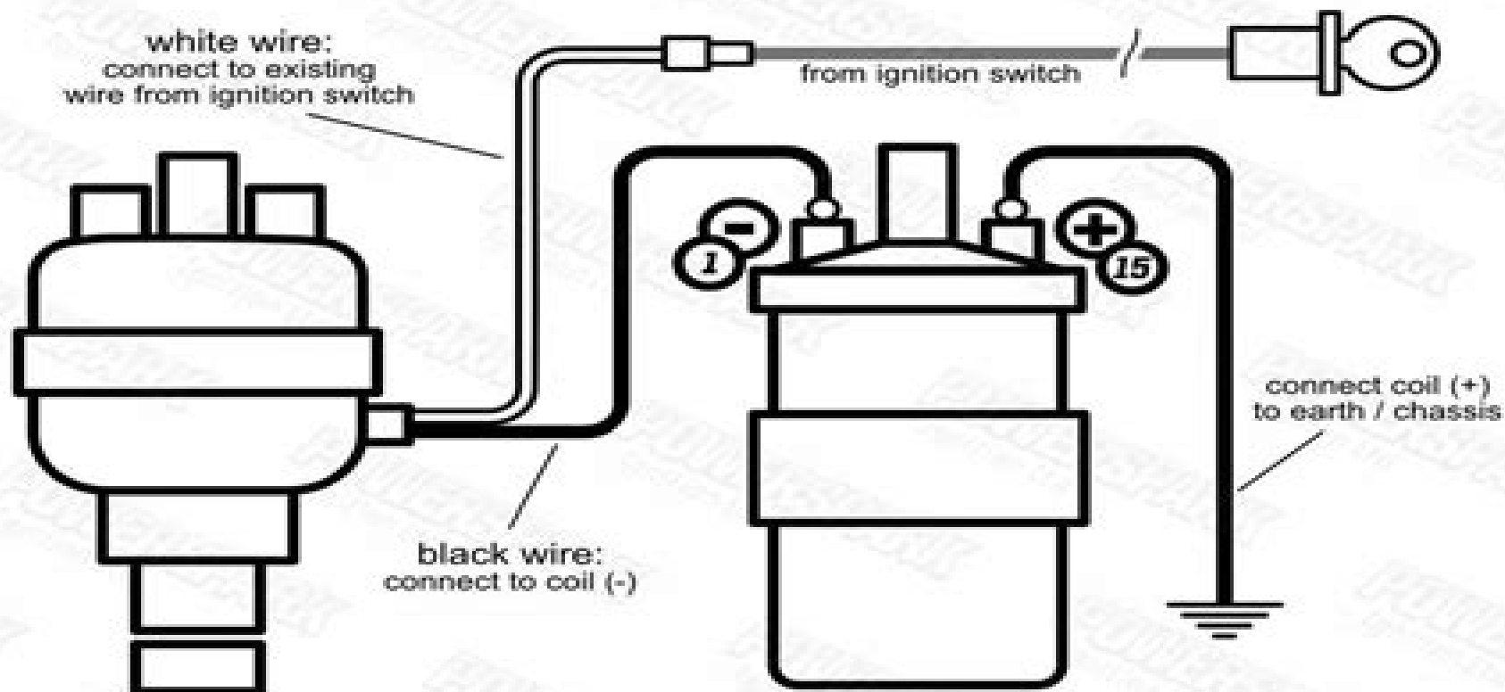
Wiring for Positive Earth Powerspark Electronic Ignition
