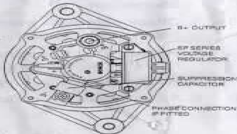
TYPICAL WIRING DIAGRAM
